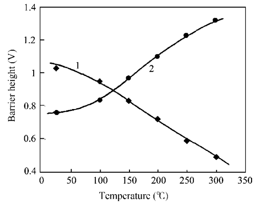
Fig. 7. Temperature dependence of Schottky barrier height of various Schottky barriers. While curve 1 is for \text{Al}_x\text{Ga}_{1-x}\text{N} diode, curve 2 is for \text{Al}_x\text{Ga}_{1-x}\text{N}/\text{GaN} diode.
