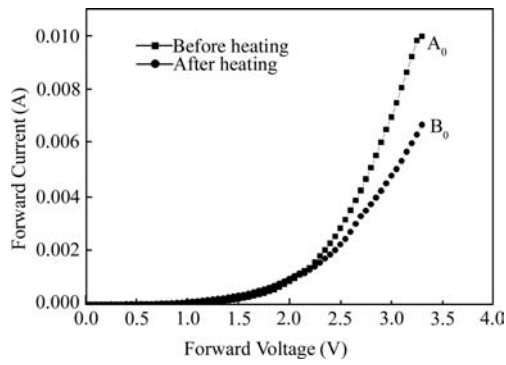
Fig. 6. Forward current–voltage characteristics of \text{Al}_x\text{Ga}_{1-x}\text{N}/\text{GaN} Schottky diodes before and after heating; curve A_0 was obtained for the diodes before heating, and curve B_0 to was obtained for the diodes after heating, both at room temperature.
