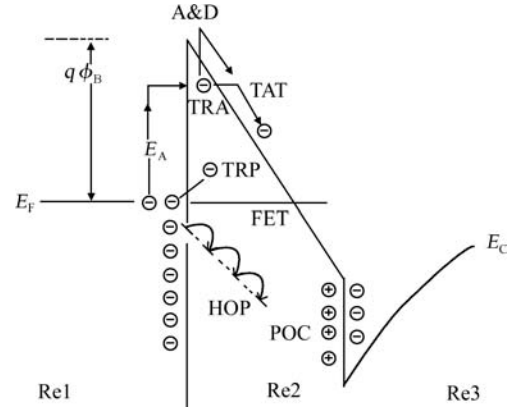
Fig. 2. Schematic diagram showing two-step trap-assisted tunneling, field-emission tunneling, trapping, hopping, in the interface regions of Al x Ga 1-x N/GaN Schottky diodes. In the figure, activation energy is denoted by E A , deep level trapping by TRP, shallow-level trapping by TRA, two-step trap-assisted tunneling by TAT, activation and drift by A&D, field-emission tunneling by FET, hopping by HOP, polarization charge by POC, metal region 1 by Re1, Al x Ga 1-x N region 2 by Re2, and GaN region 3 by Re3.
