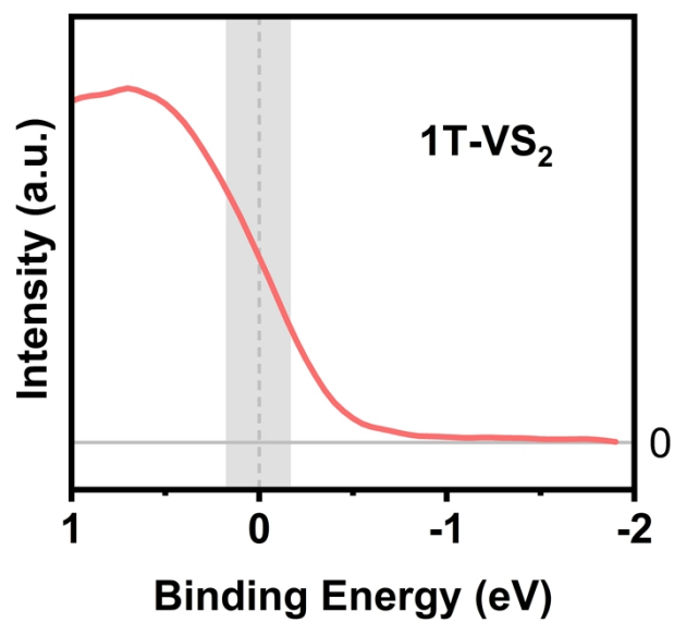
Figure S1 The valence band X-ray photoelectron spectroscopy (VB XPS) of 1T-VS 2 .
