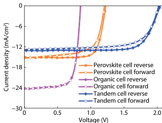
Fig. S7. (Color online) J - V curves for the single-junction perovskite cell, single-junction organic cell, and tandem cell under forward and reverse scans.
