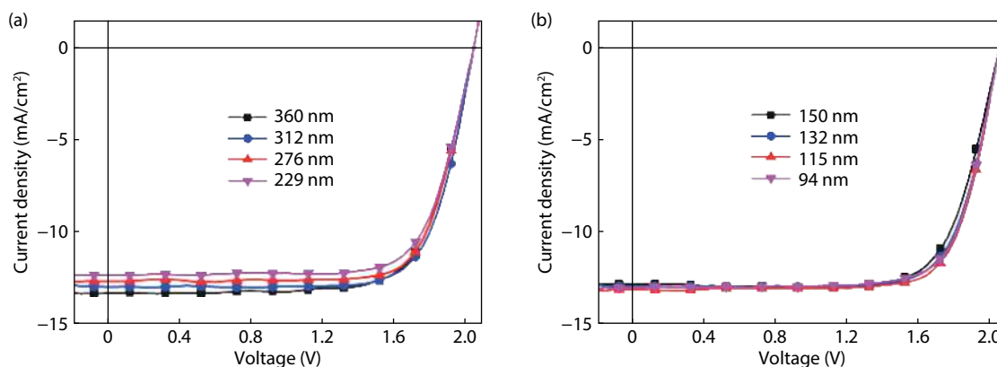
Fig. S6. (Color online) (a) J - V curves for the tandem cells changing with the thickness of the CsPbI 2 Br layer (thickness of D18:Y6 layer: 132 nm). (b) J - V curves for the tandem cells changing with the thickness of the D18:Y6 layer (thickness of CsPbI 2 Br layer: 312 nm).
