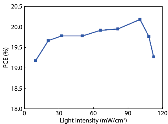
Fig. S9. PCE for the tandem cell under different light intensities.
