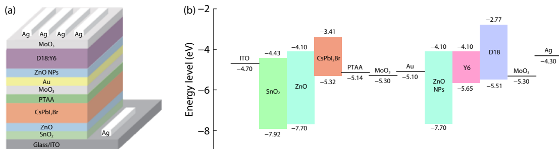
Fig. S4. (Color online) (a) Structure of the tandem cell. (b) Energy level diagram.
