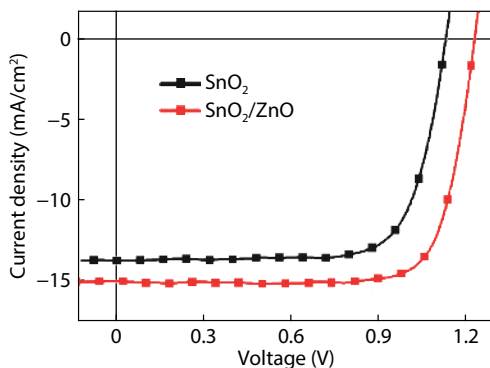
Fig. S2. (Color online) J - V curves for single-junction perovskite solar cells with different electron-transport layer.
