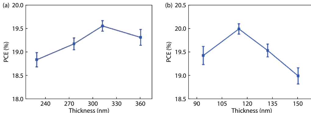
Fig. S5. (a) PCE for tandem cells changing with the thickness of the CsPbI 2 Br layer (the thickness of D18:Y6 layer: 132 nm). (b) PCE for tandem cells changing with the thickness of the D18:Y6 layer (the thickness of CsPbI 2 Br layer: 312 nm).
