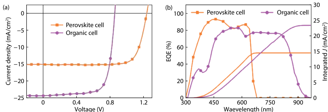
Fig. S3. (Color online) (a) J - V curves for the single-junction perovskite ( \text{CsPbI}_2\text{Br} ) cell and organic (D18:Y6) cell; (b) EQE spectra for the cells.
