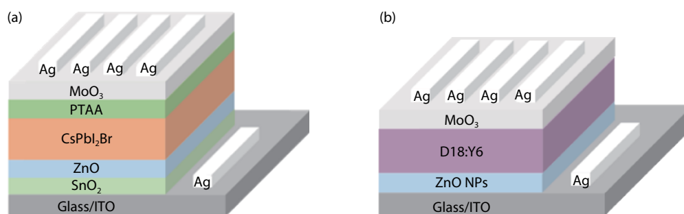
Fig. S1. (Color online) The structures for the (a) single-junction perovskite cells and organic (b) cells.
