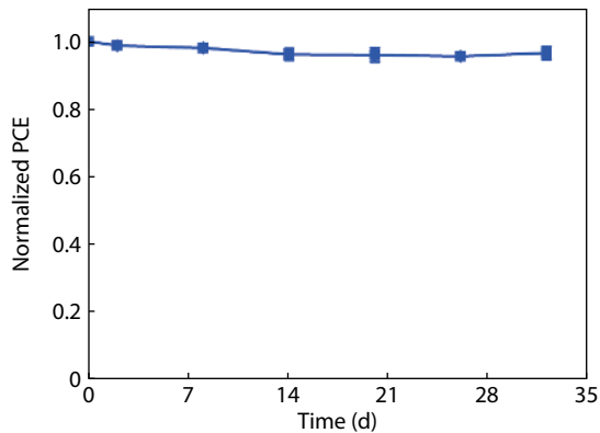
Fig. S10. PCE change for tandem cells stored in \text{N}_2 glovebox.
